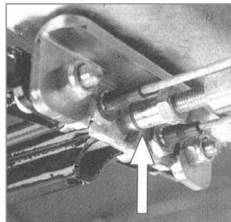
Locate ATC on the axle and check to position of the push rod. (See photograph above).
