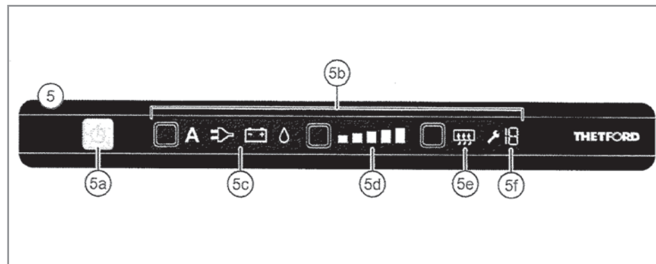
Control Panel with touchscreen
