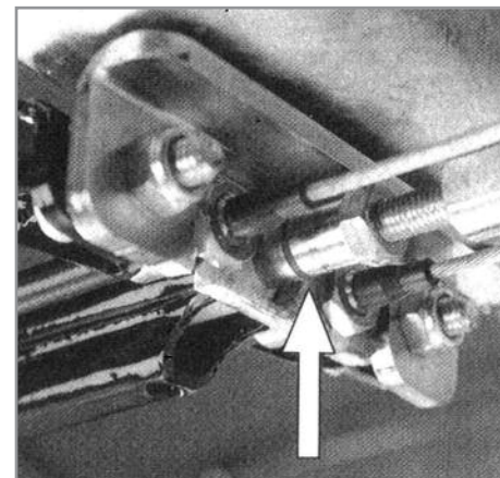
Locate ATC on the axle and check to position of the push rod. (See photograph).
